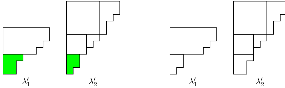
FIGURE 2. Illustration of the 4-conjugation (see Example 1). For the initial overpartition \pi (on the left), we have \lambda'_1 = (7, 7, 6, 5, 3, 2, 2) and \lambda'_2 = (8, 8, 7, 6, 6, 5, 4, 3, 2, 2, 1) . The regions highlighted are interchanged by 4-conjugation, which gives \lambda'_1 = (7, 7, 6, 5, 2, 2, 1) and \lambda'_2 = (8, 8, 7, 6, 6, 5, 4, 3, 3, 2, 2) for \pi^{(4)} , the 4-conjugate of \pi (on the right).
