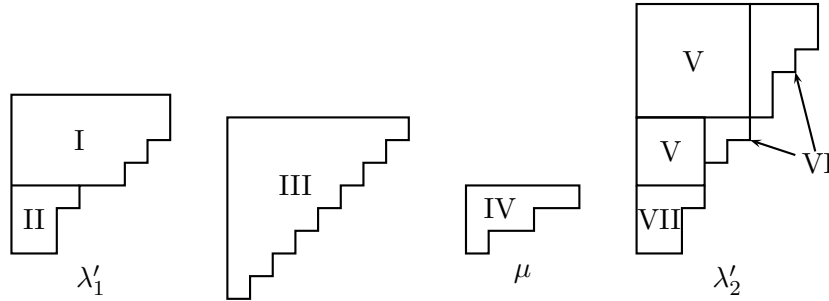
FIGURE 3. Decomposition of a self- k -conjugate overpartition (in this example, k = 4 ).
